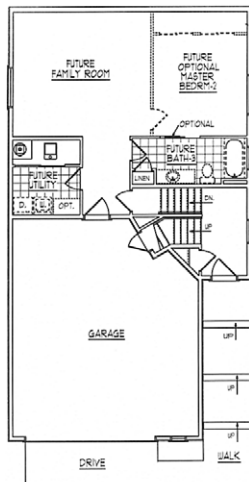
FUTURE FINISHED LOWER FLOOR PLAN
